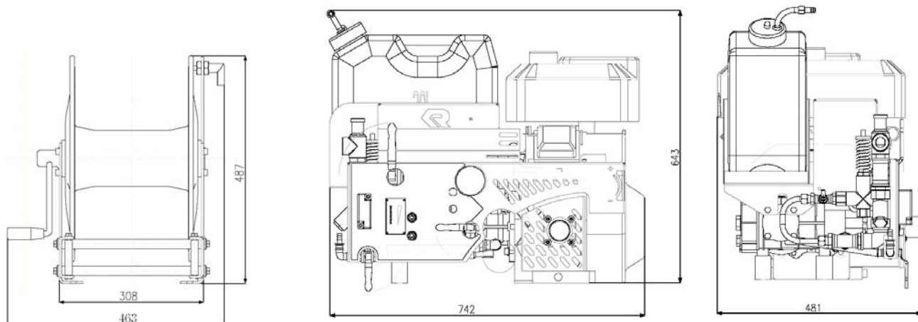
Dimensions of hose reel and basic module (in mm)
