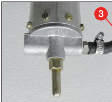
Bottom pin for quick and easy fitting onto a tripod or vehicle mounting bracket
