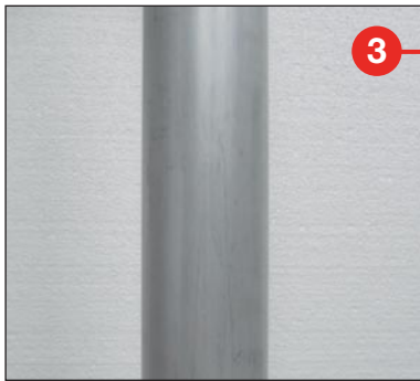
Standard natural clear anodised seamless drawn aluminium mast sections with Ø 2 1/2" (63,5 mm) base tube
